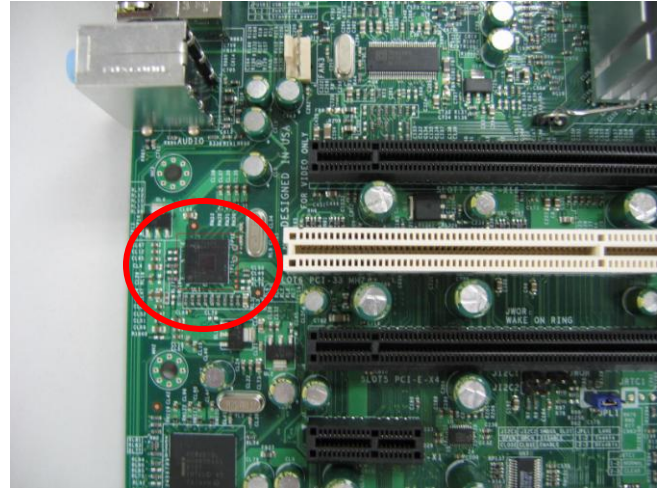
Photo of board with LAN heatsink removed
