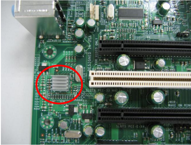
Photo of board with LAN heatsink installed
